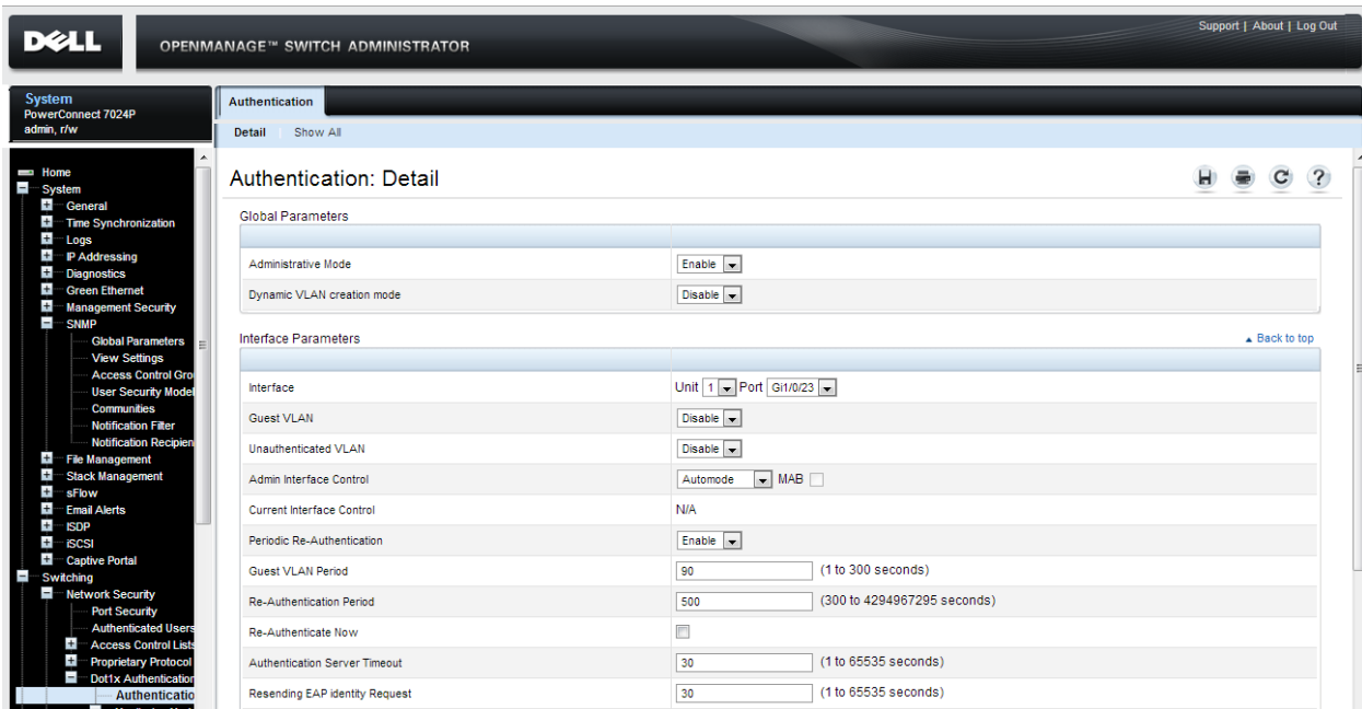
Figure 12. OnGuard 7024P Switch - Authentication Configuration
