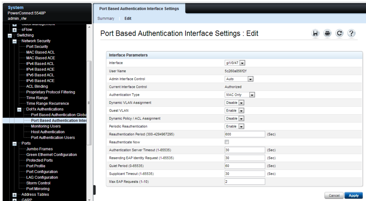
Figure 25. Appendix A, 5524P Dot1x Interface Settings, MAC Only
